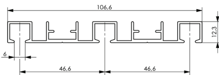
Objektschiene, Art. A-380-3W object rail
