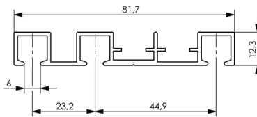
Objektschiene, Art. A-370-3 object rail
