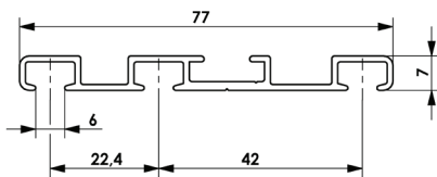
Objektschiene, Art. A-390-3 object rail
