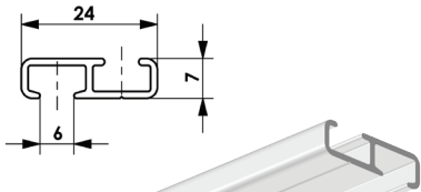
Objektschiene, Art. A-388-1 object rail
